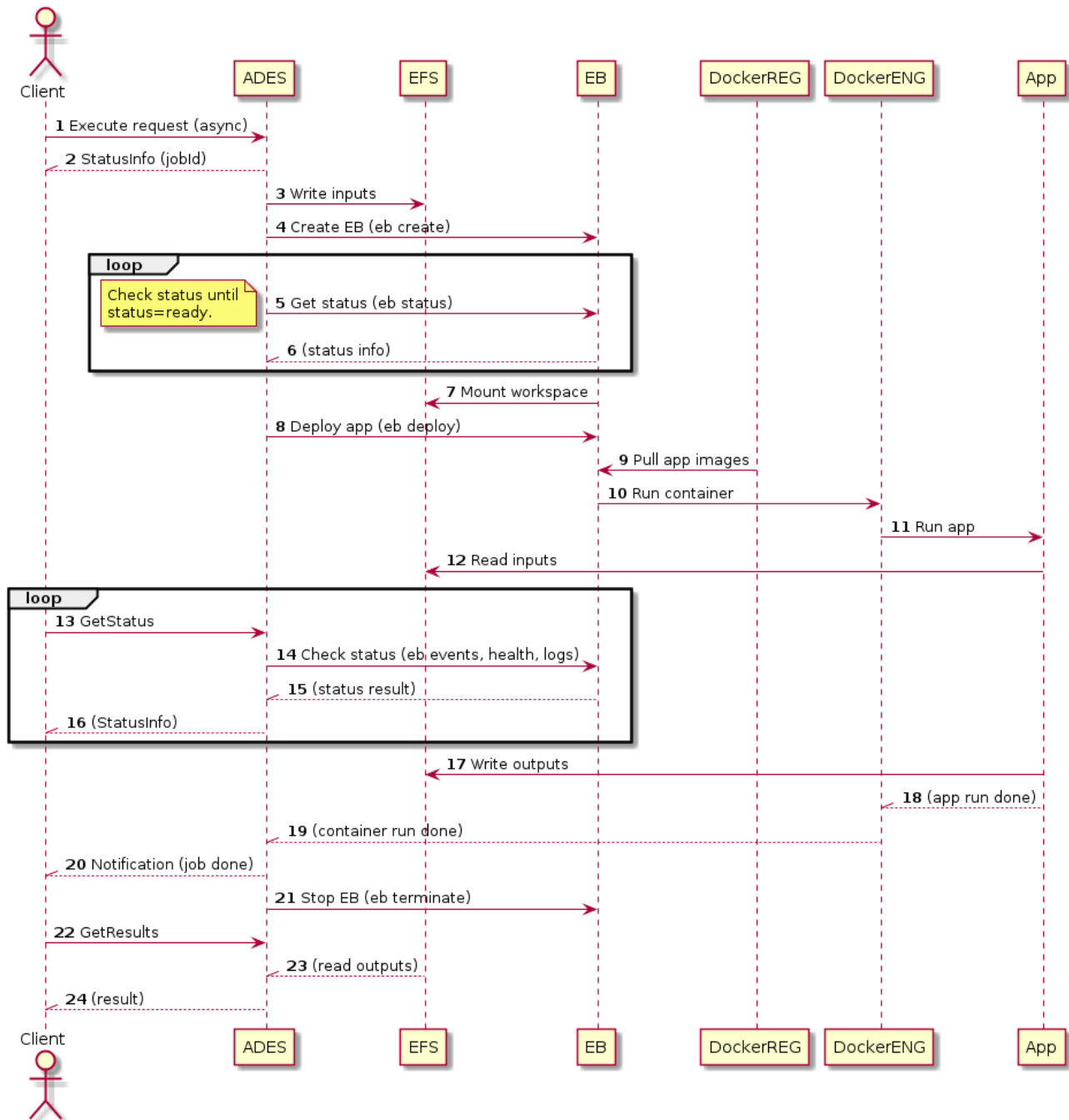
Figure 14. Sequence Diagram for Application Execution
