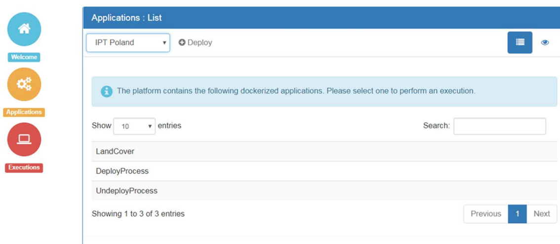
Figure 18. Applications Screen
