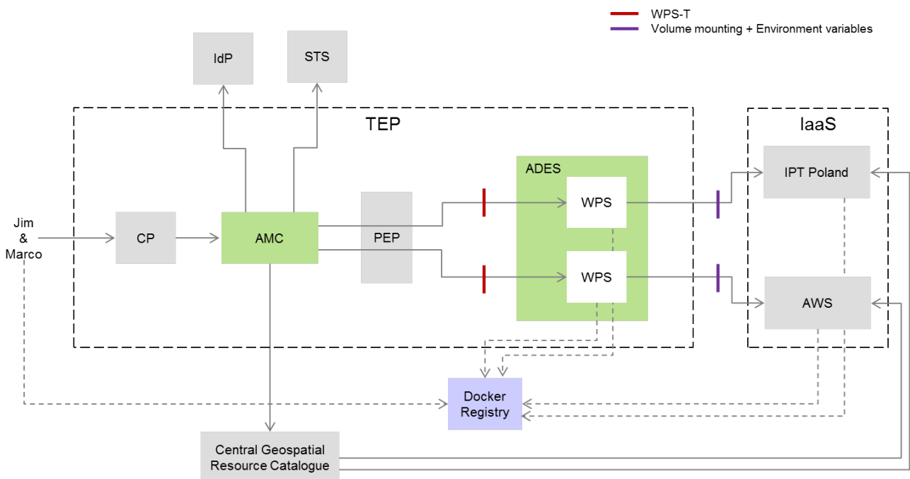
Figure 15. Alternative Approach Overview
