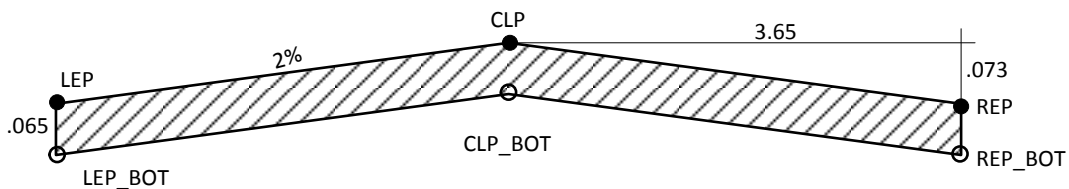
Figure 13. Pavement CrossSectionComponent
